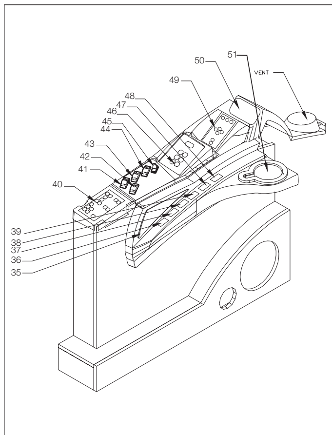
Shifter Selector (Side-Pod)
